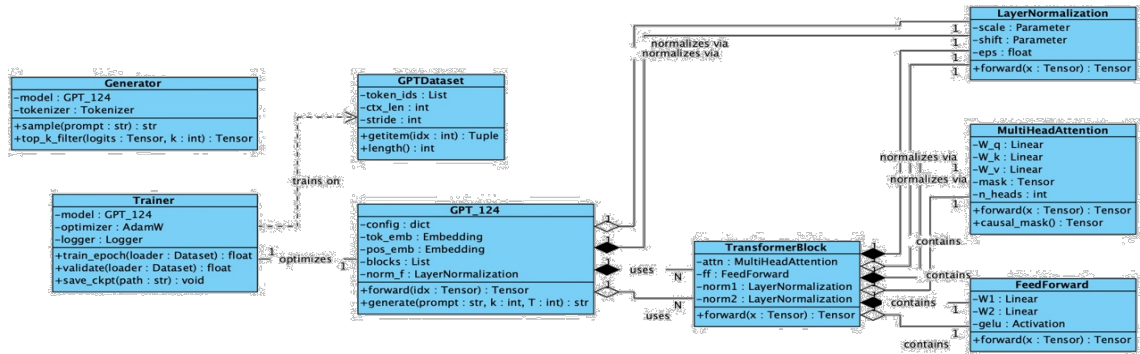
Figure 6: Class Diagram
